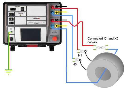
Connecting TRT400 to an unmounted current transformer
