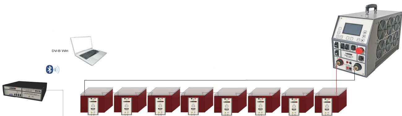
Connectivity diagram of BVS system components in combination with Battery Load Unit device
